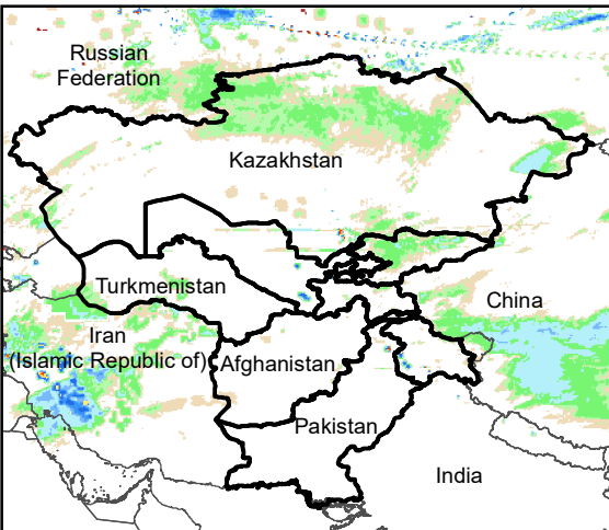
Daily Rainfall estimate for 10 Jan., 2005
