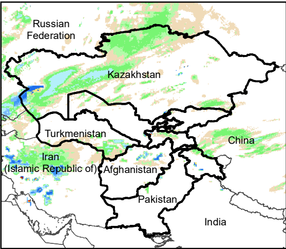
Daily Rainfall estimate for 9 Jan., 2005
