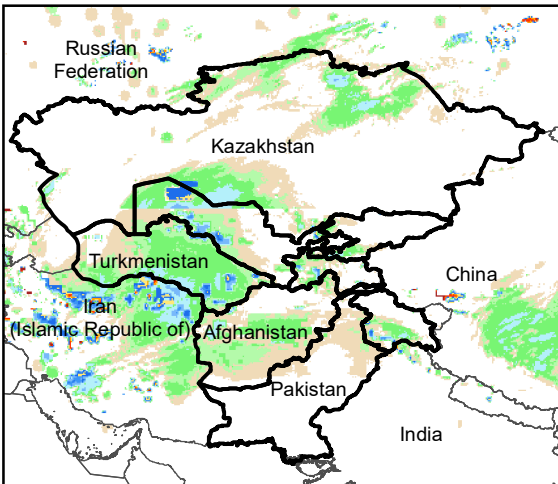
Daily Rainfall estimate for 11 Jan., 2005
