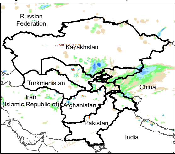
Daily Rainfall estimate for 14 Jan., 2005
