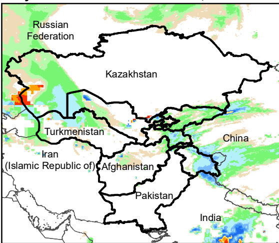
Daily Rainfall estimate for 2 Feb., 2005
