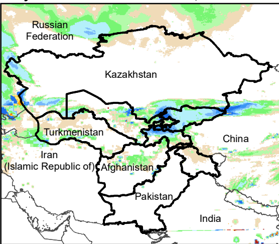
Daily Rainfall estimate for 4 Feb., 2005
