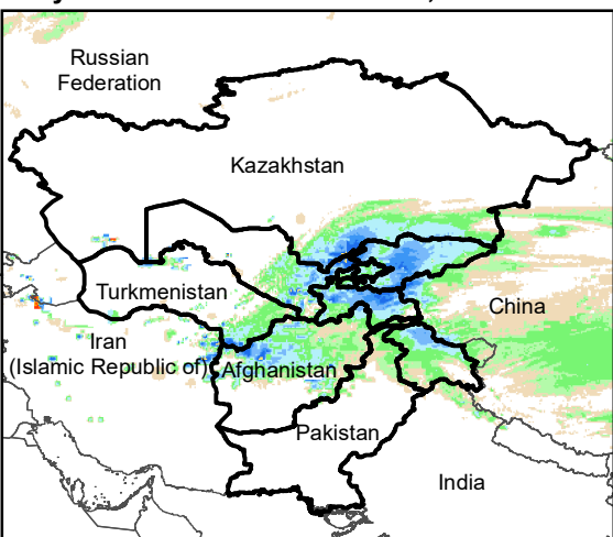
Daily Rainfall estimate for 3 Feb., 2005
