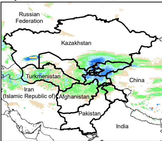
Daily Rainfall estimate for 5 Feb., 2005
