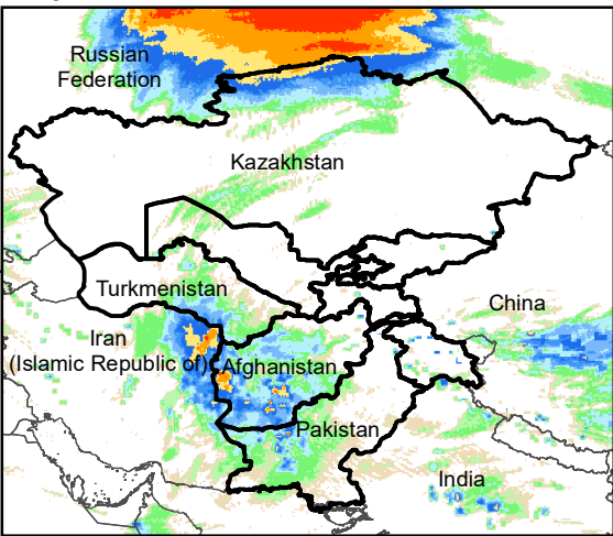
Daily Rainfall estimate for 6 Mar., 2005
