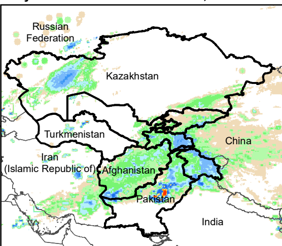
Daily Rainfall estimate for 17 Mar., 2005
