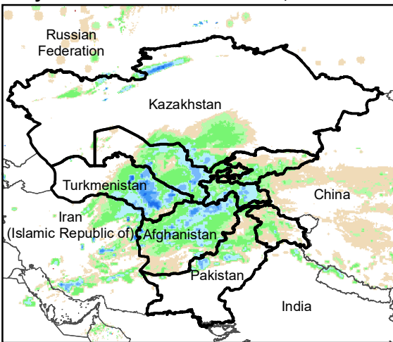
Daily Rainfall estimate for 18 Mar., 2005
