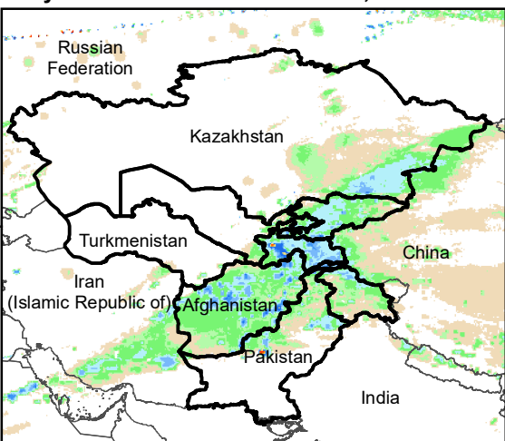
Daily Rainfall estimate for 16 Mar., 2005
