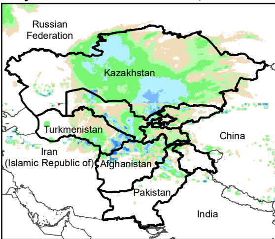
Daily Rainfall estimate for 28 Mar., 2005
