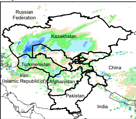
Daily Rainfall estimate for 27 Mar., 2005
