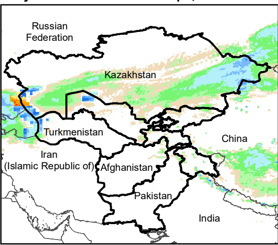
Daily Rainfall estimate for 1 Apr., 2005
