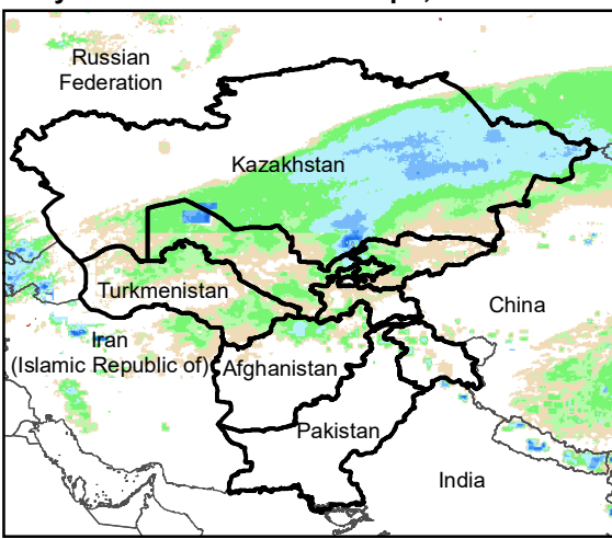
Daily Rainfall estimate for 3 Apr., 2005
