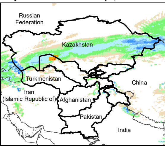
Daily Rainfall estimate for 2 Apr., 2005
