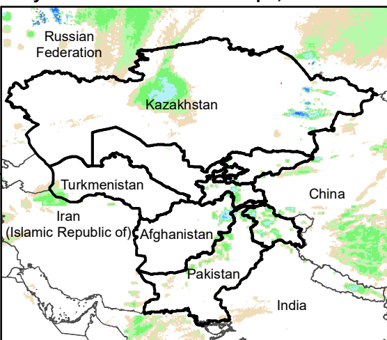
Daily Rainfall estimate for 21 Apr., 2005
