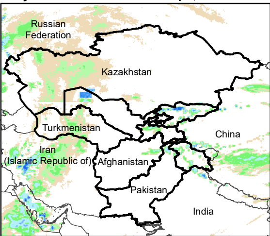
Daily Rainfall estimate for 20 Apr., 2005
