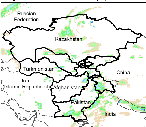
Daily Rainfall estimate for 22 Apr., 2005
