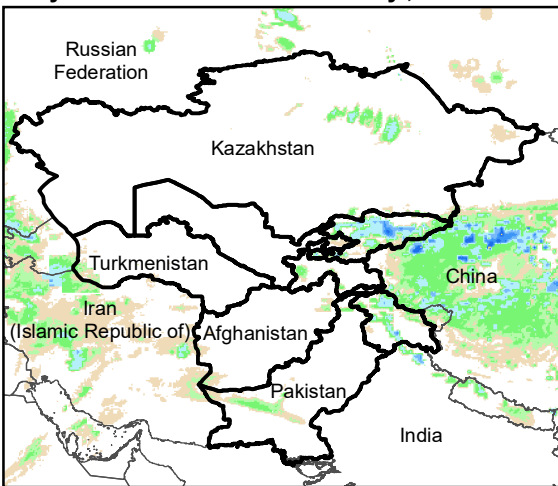
Daily Rainfall estimate for 17 May., 2005
