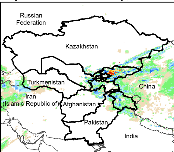
Daily Rainfall estimate for 16 May., 2005
