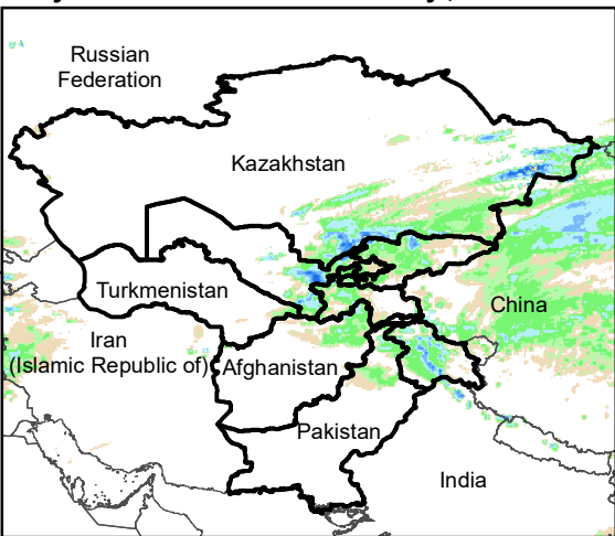
Daily Rainfall estimate for 15 May., 2005
