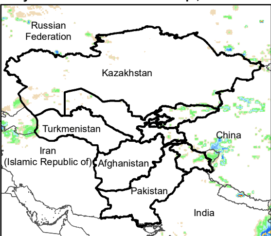
Daily Rainfall estimate for 30 Sep., 2005
