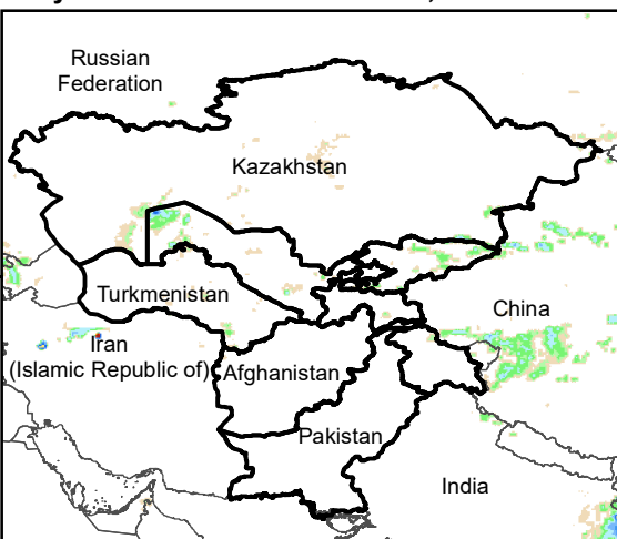
Daily Rainfall estimate for 1 Oct., 2005
