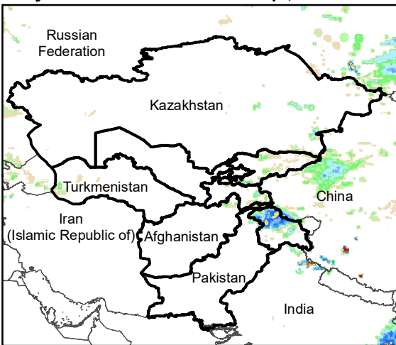
Daily Rainfall estimate for 2 Oct., 2005
