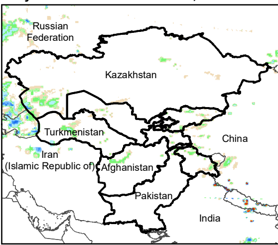
Daily Rainfall estimate for 5 Oct., 2005
