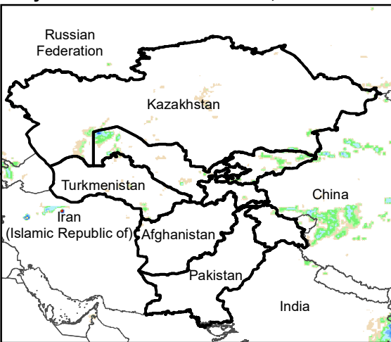
Daily Rainfall estimate for 4 Oct., 2005
