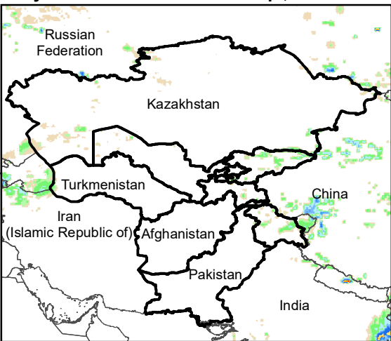
Daily Rainfall estimate for 3 Oct., 2005
