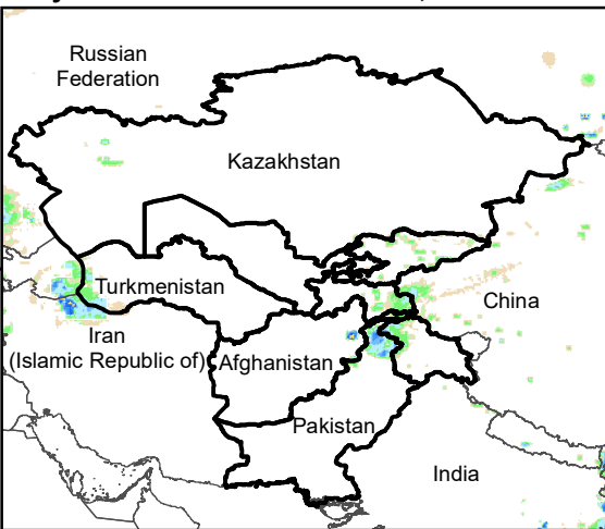
Daily Rainfall estimate for 7 Oct., 2005
