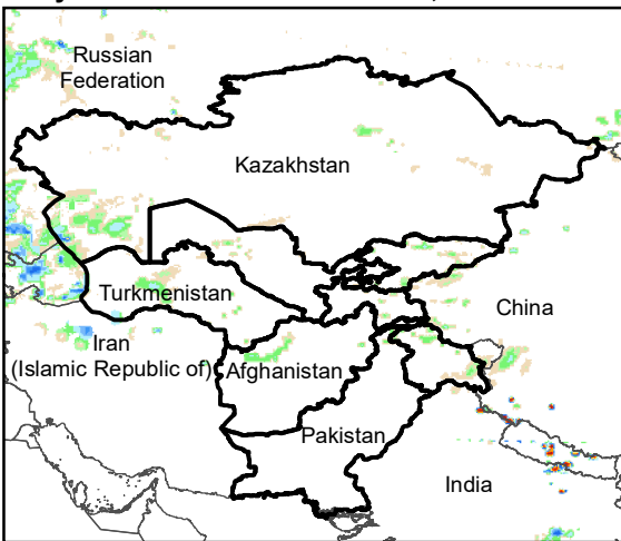
Daily Rainfall estimate for 8 Oct., 2005
