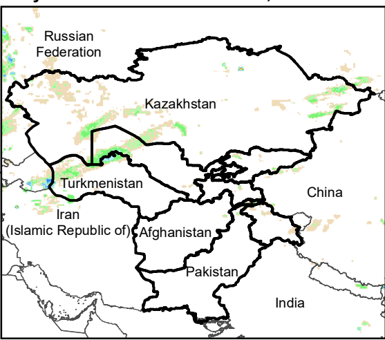
Daily Rainfall estimate for 6 Oct., 2005
