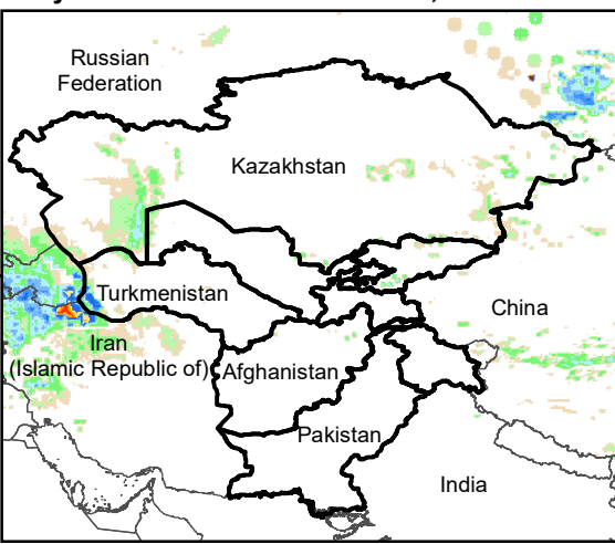
Daily Rainfall estimate for 5 Nov., 2005
