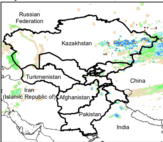
Daily Rainfall estimate for 6 Nov., 2005
