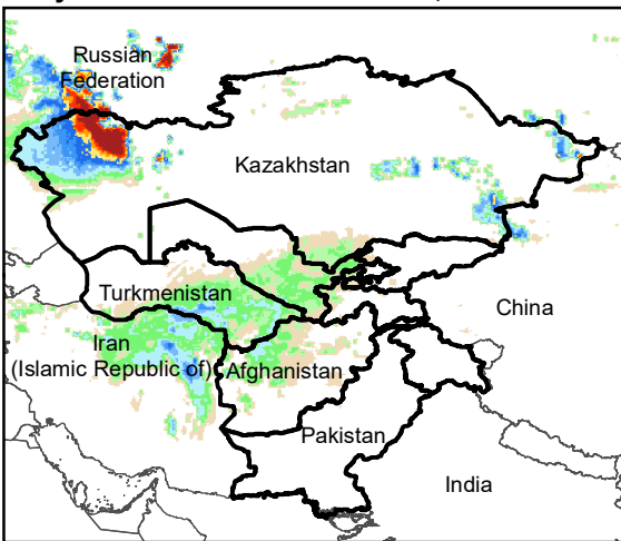
Daily Rainfall estimate for 12 Nov., 2005
