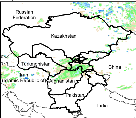
Daily Rainfall estimate for 10 Nov., 2005
