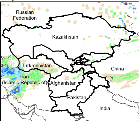
Daily Rainfall estimate for 11 Nov., 2005
