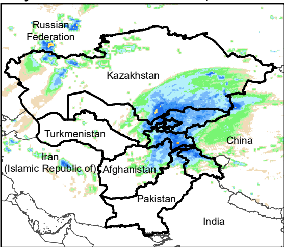
Daily Rainfall estimate for 13 Nov., 2005
