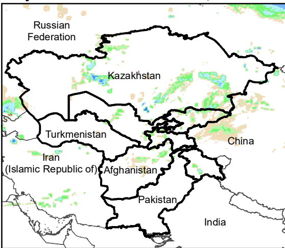
Daily Rainfall estimate for 15 Nov., 2005
