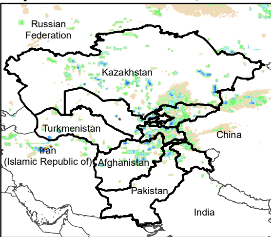
Daily Rainfall estimate for 14 Nov., 2005
