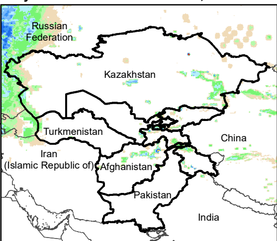
Daily Rainfall estimate for 30 Nov., 2005
