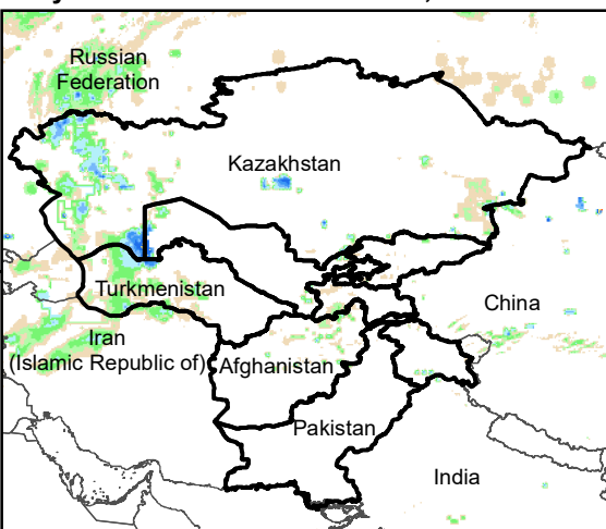
Daily Rainfall estimate for 1 Dec., 2005
