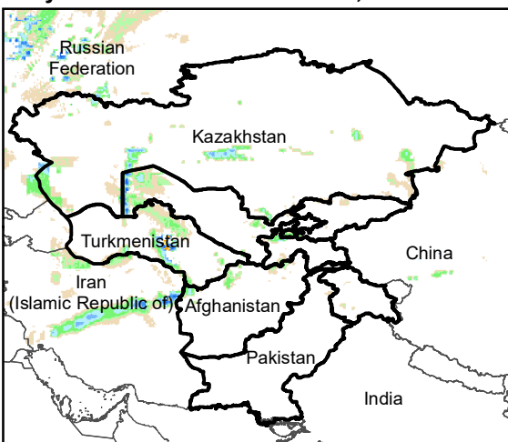
Daily Rainfall estimate for 2 Dec., 2005
