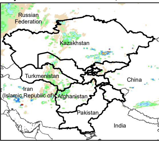
Daily Rainfall estimate for 18 Dec., 2005
