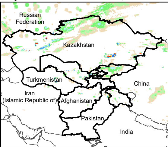
Daily Rainfall estimate for 17 Dec., 2005
