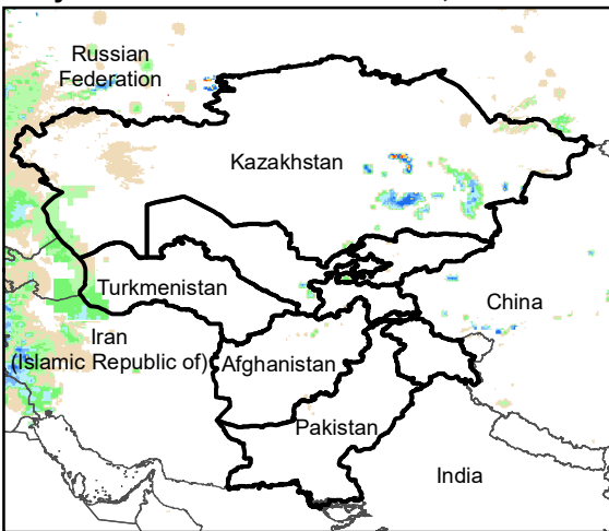
Daily Rainfall estimate for 19 Dec., 2005
