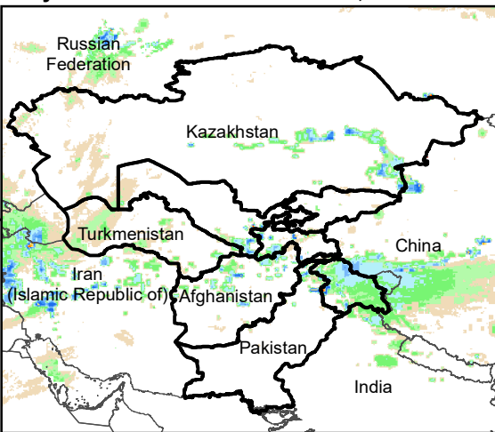
Daily Rainfall estimate for 18 Feb., 2006
