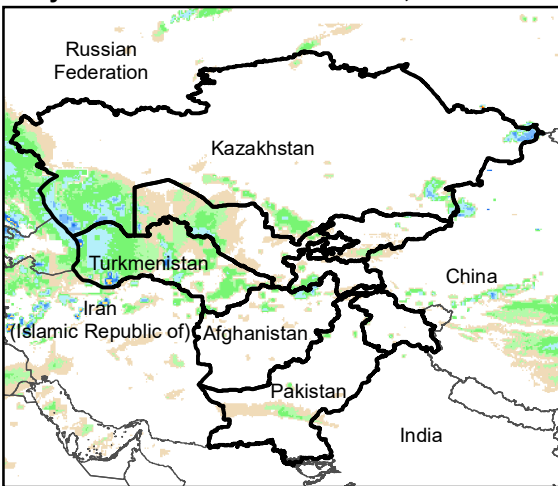
Daily Rainfall estimate for 19 Feb., 2006
