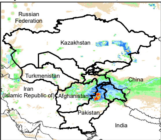
Daily Rainfall estimate for 17 Feb., 2006
