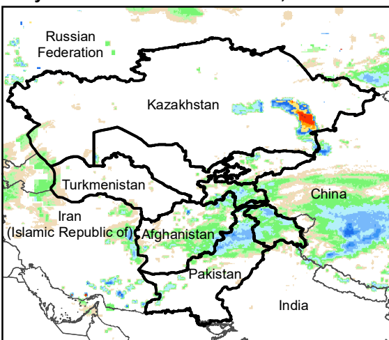
Daily Rainfall estimate for 19 Mar., 2006
