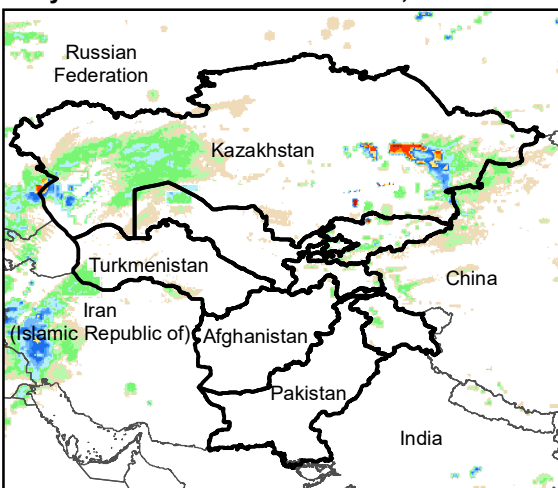
Daily Rainfall estimate for 30 Oct., 2006
