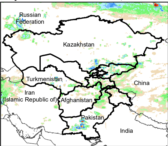
Daily Rainfall estimate for 28 Oct., 2006
