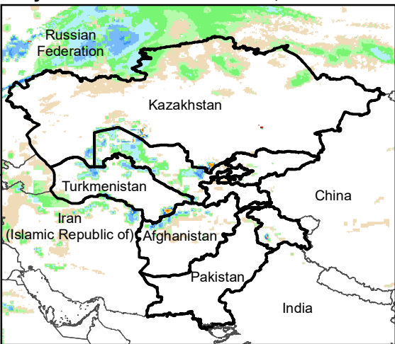
Daily Rainfall estimate for 8 Jan., 2007
