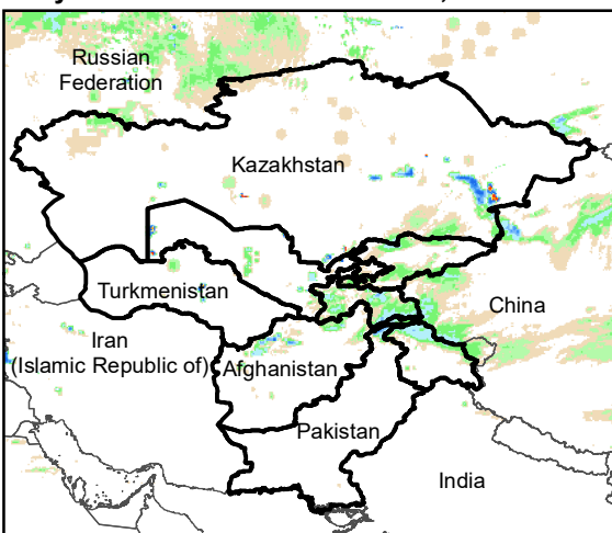
Daily Rainfall estimate for 11 Jan., 2007
