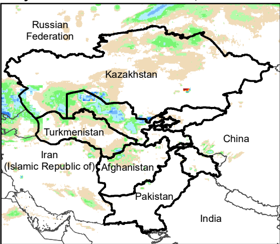
Daily Rainfall estimate for 9 Jan., 2007
