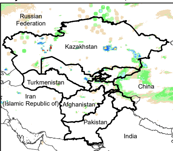
Daily Rainfall estimate for 10 Jan., 2007
