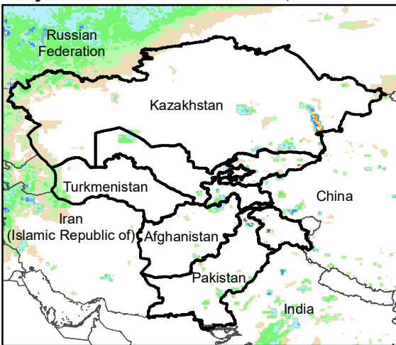
Daily Rainfall estimate for 1 Feb., 2007
