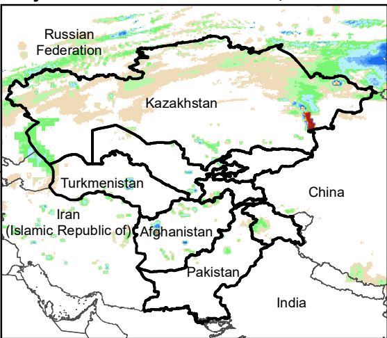
Daily Rainfall estimate for 30 Jan., 2007
