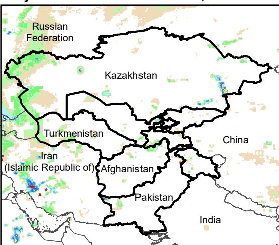
Daily Rainfall estimate for 31 Jan., 2007
