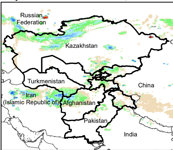
Daily Rainfall estimate for 20 Feb., 2007
