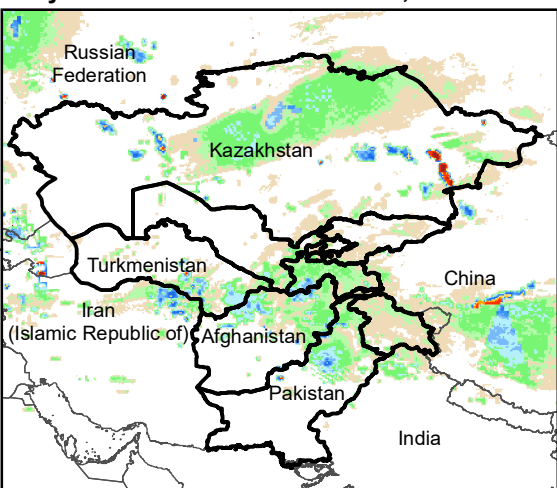
Daily Rainfall estimate for 18 Feb., 2007
