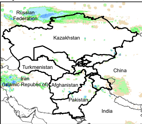
Daily Rainfall estimate for 19 Feb., 2007
