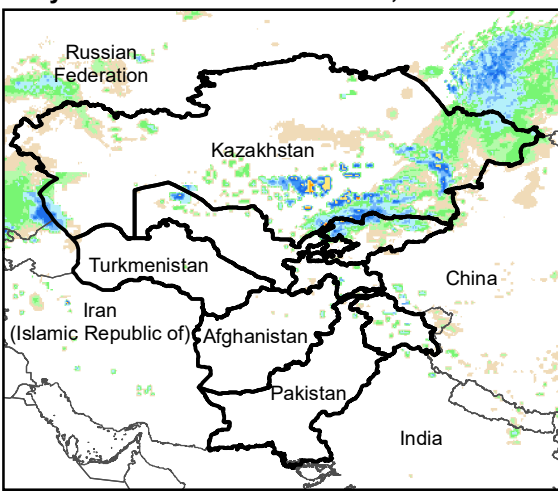
Daily Rainfall estimate for 9 Nov., 2007
