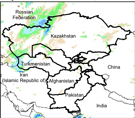
Daily Rainfall estimate for 7 Nov., 2007
