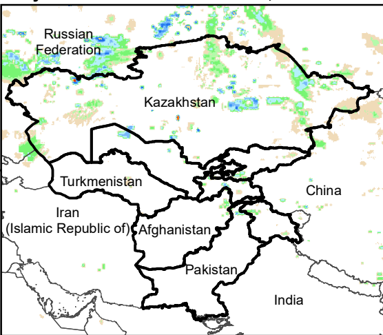
Daily Rainfall estimate for 8 Nov., 2007
