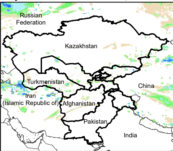
Daily Rainfall estimate for 28 Nov., 2007
