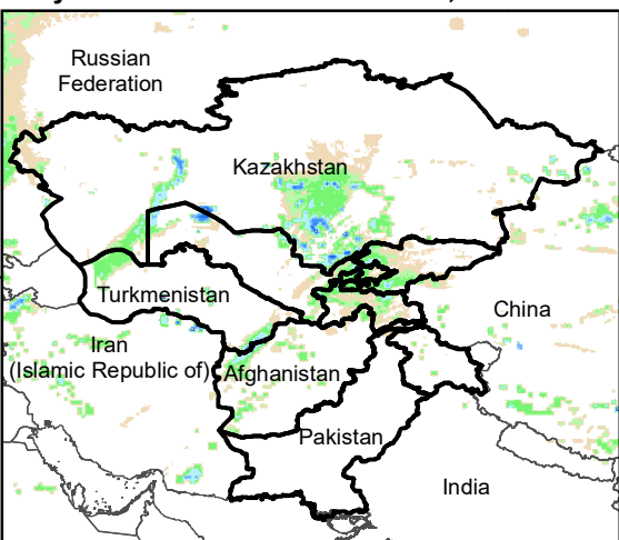
Daily Rainfall estimate for 27 Nov., 2007
