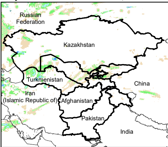
Daily Rainfall estimate for 29 Nov., 2007
