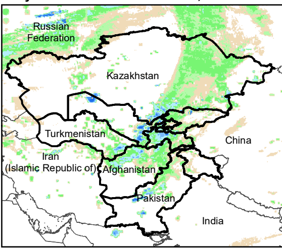
Daily Rainfall estimate for 1 Dec., 2007
