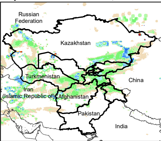
Daily Rainfall estimate for 6 Jan., 2008
