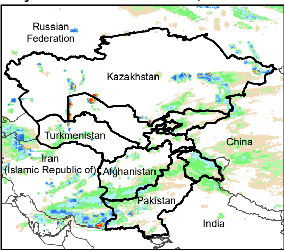
Daily Rainfall estimate for 5 Jan., 2008
