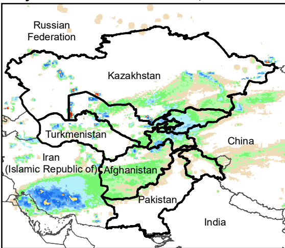
Daily Rainfall estimate for 7 Jan., 2008
