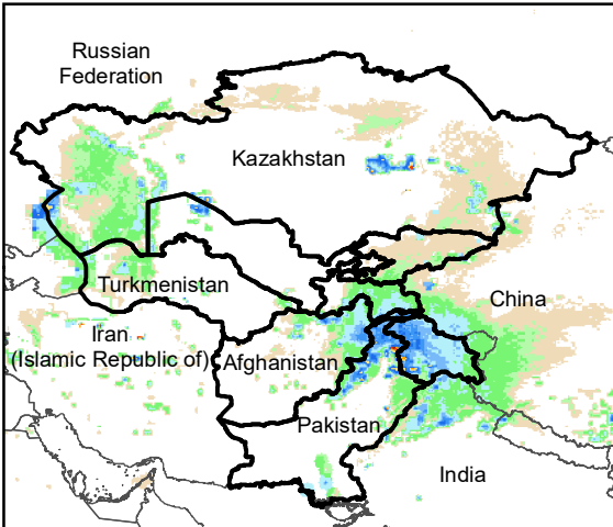
Daily Rainfall estimate for 9 Jan., 2008
