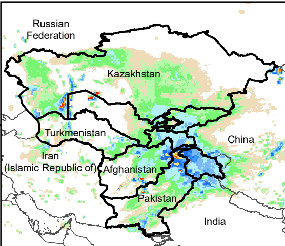
Daily Rainfall estimate for 8 Jan., 2008
