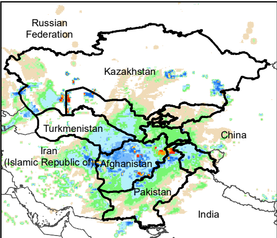
Daily Rainfall estimate for 7 Jan., 2008
