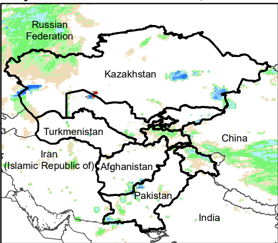
Daily Rainfall estimate for 31 Jan., 2008
