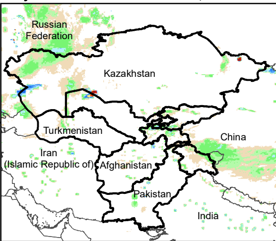
Daily Rainfall estimate for 1 Feb., 2008
