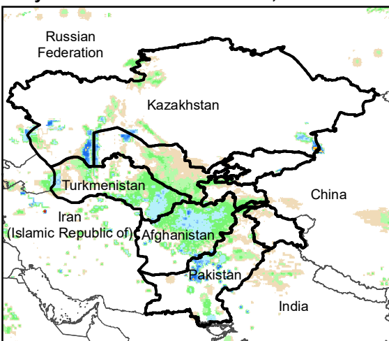
Daily Rainfall estimate for 2 Feb., 2008
