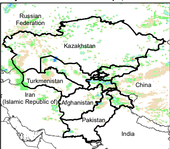
Daily Rainfall estimate for 19 Apr., 2008
