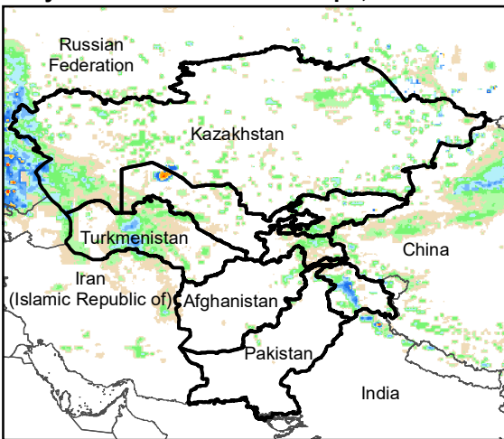
Daily Rainfall estimate for 21 Apr., 2008
