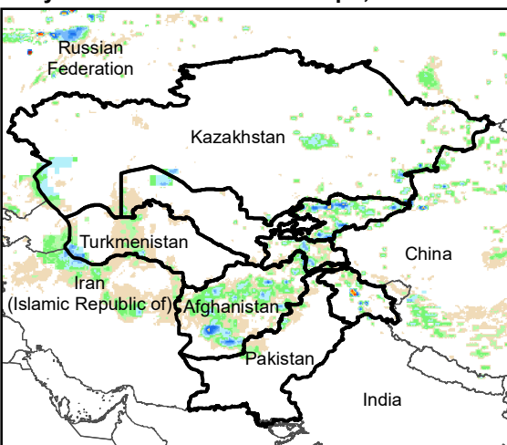
Daily Rainfall estimate for 20 Apr., 2008
