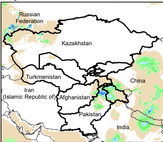
Daily Rainfall estimate for 10 Oct., 2008
