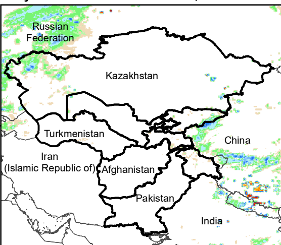
Daily Rainfall estimate for 9 Oct., 2008
