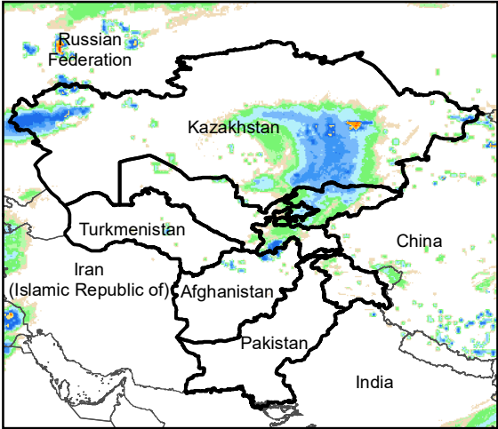
Daily Rainfall estimate for 27 Oct., 2008
