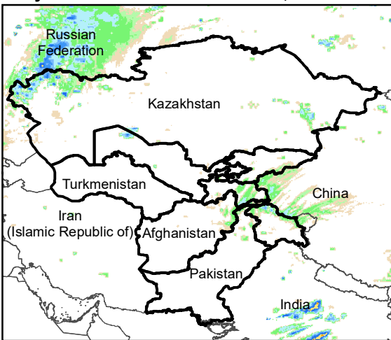
Daily Rainfall estimate for 22 Nov., 2008
