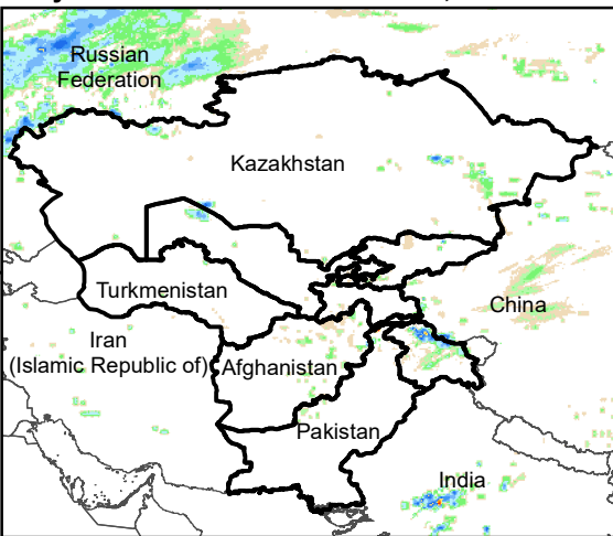
Daily Rainfall estimate for 21 Nov., 2008
