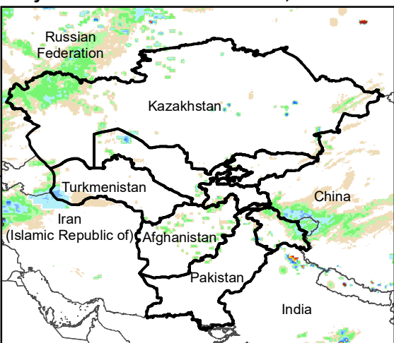
Daily Rainfall estimate for 20 Nov., 2008
