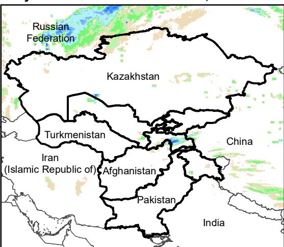
Daily Rainfall estimate for 25 Nov., 2008
