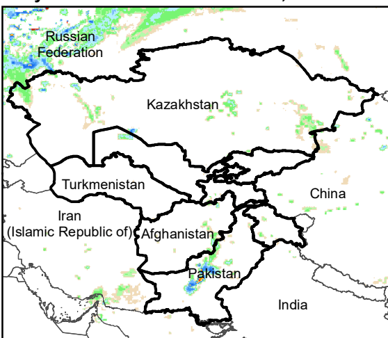
Daily Rainfall estimate for 27 Nov., 2008
