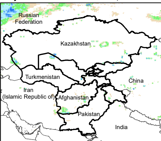
Daily Rainfall estimate for 26 Nov., 2008
