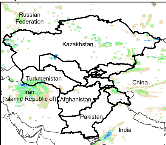
Daily Rainfall estimate for 4 Dec., 2008
