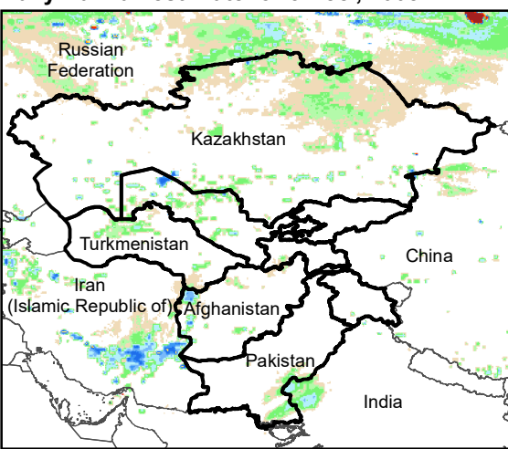
Daily Rainfall estimate for 5 Dec., 2008
