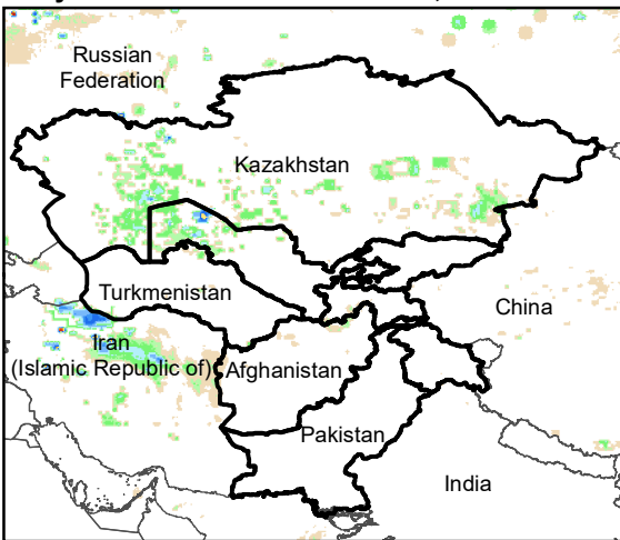
Daily Rainfall estimate for 6 Dec., 2008
