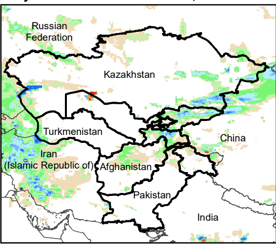
Daily Rainfall estimate for 4 Feb., 2010
