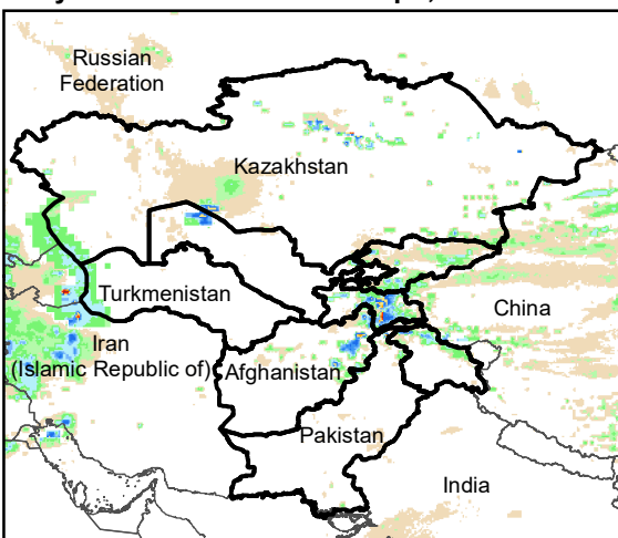
Daily Rainfall estimate for 8 Apr., 2010
