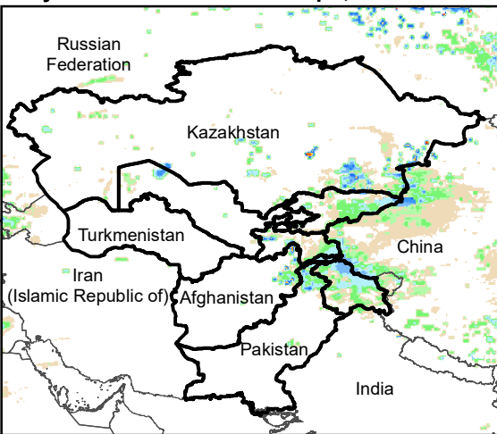
Daily Rainfall estimate for 7 Apr., 2010
