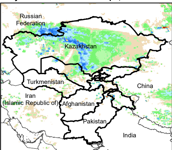
Daily Rainfall estimate for 6 Apr., 2010
