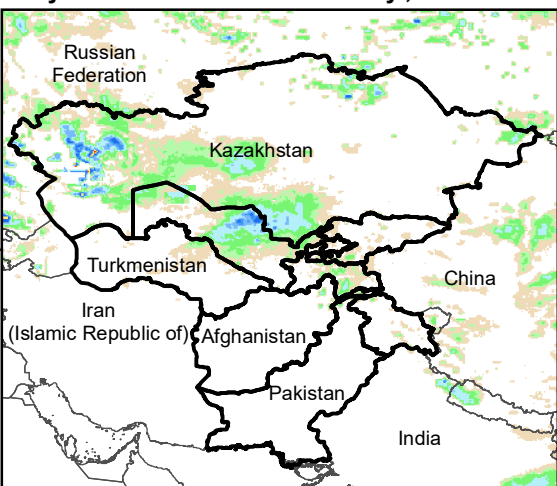
Daily Rainfall estimate for 25 May., 2010
