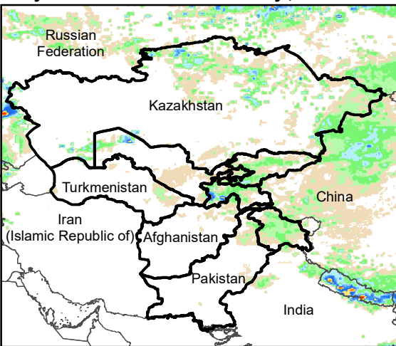
Daily Rainfall estimate for 26 May., 2010
