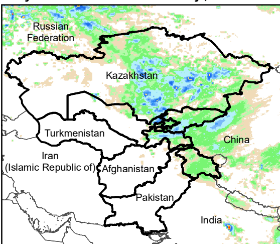
Daily Rainfall estimate for 27 May., 2010
