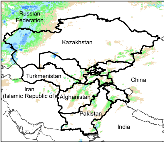
Daily Rainfall estimate for 29 Oct., 2010
