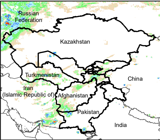
Daily Rainfall estimate for 28 Oct., 2010
