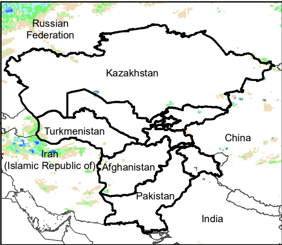
Daily Rainfall estimate for 27 Oct., 2010
