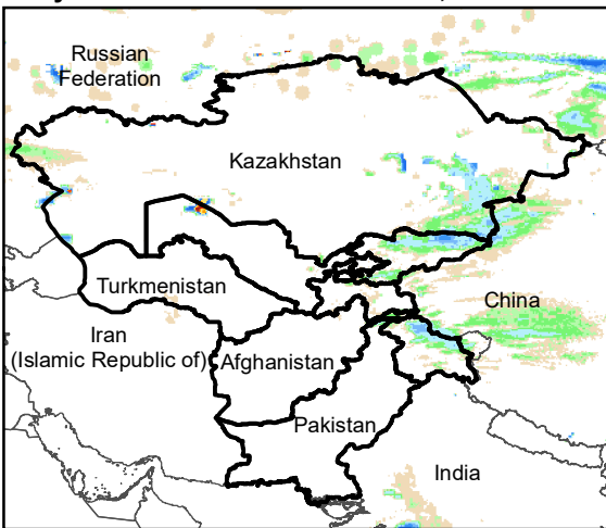
Daily Rainfall estimate for 24 Nov., 2010
