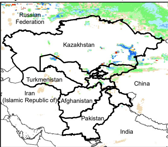
Daily Rainfall estimate for 23 Nov., 2010
