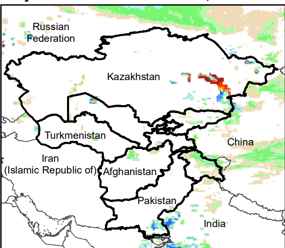
Daily Rainfall estimate for 22 Nov., 2010
