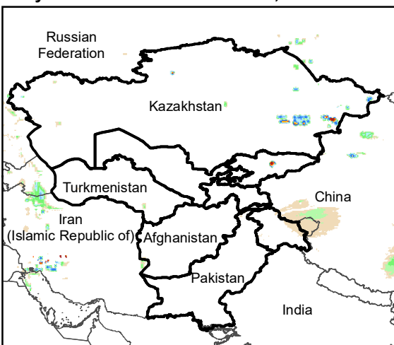
Daily Rainfall estimate for 8 Jan., 2011
