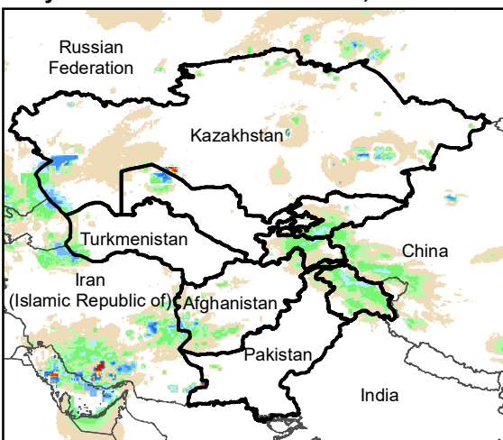
Daily Rainfall estimate for 28 Jan., 2011
