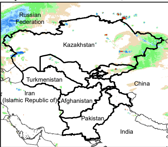
Daily Rainfall estimate for 27 Jan., 2011
