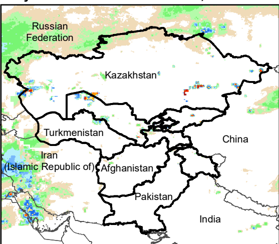
Daily Rainfall estimate for 26 Jan., 2011
