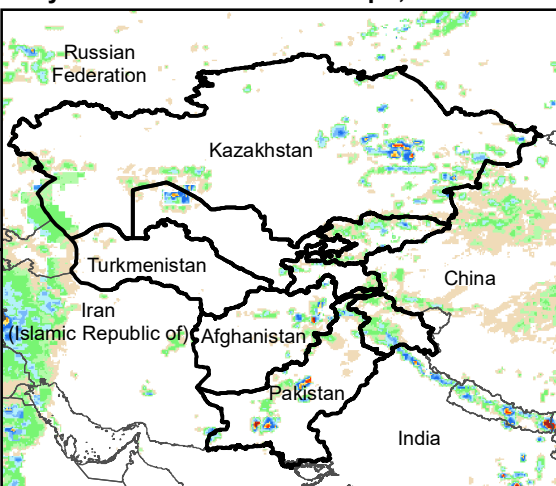
Daily Rainfall estimate for 30 Apr., 2011
