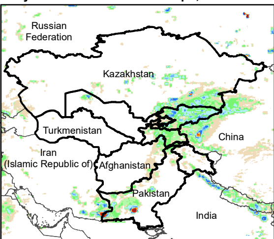
Daily Rainfall estimate for 29 Apr., 2011
