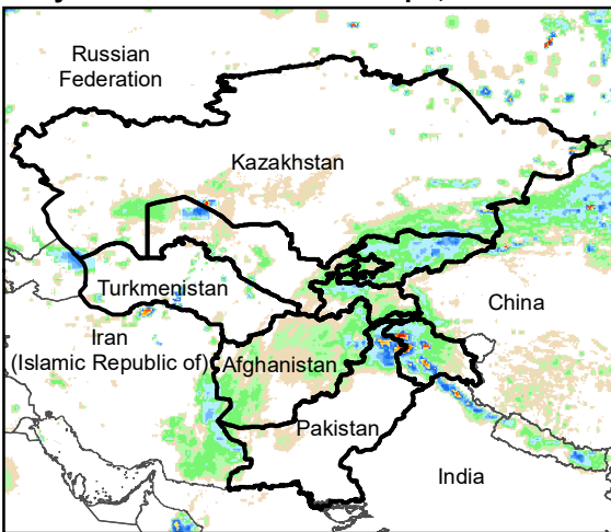
Daily Rainfall estimate for 1 May., 2011
