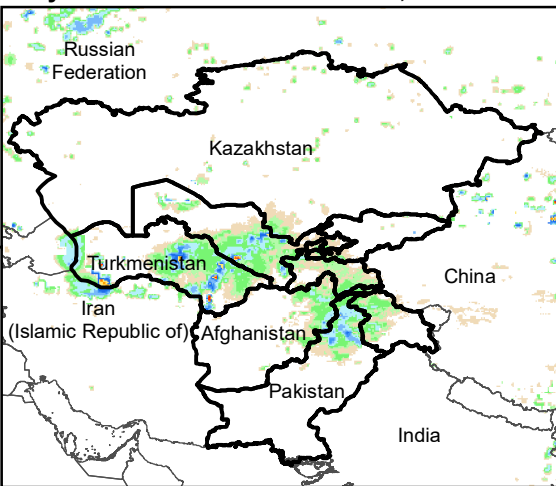
Daily Rainfall estimate for 25 Oct., 2011
