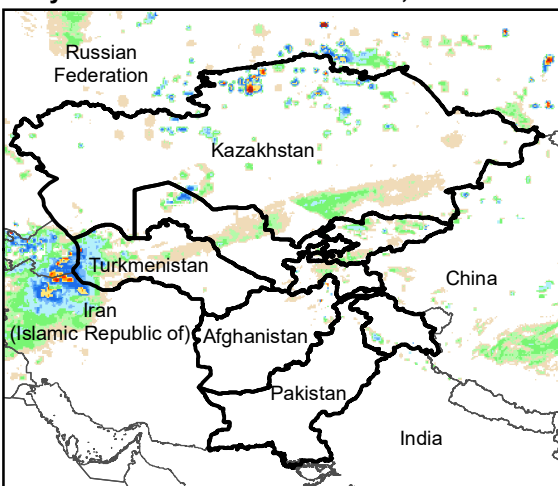
Daily Rainfall estimate for 26 Oct., 2011
