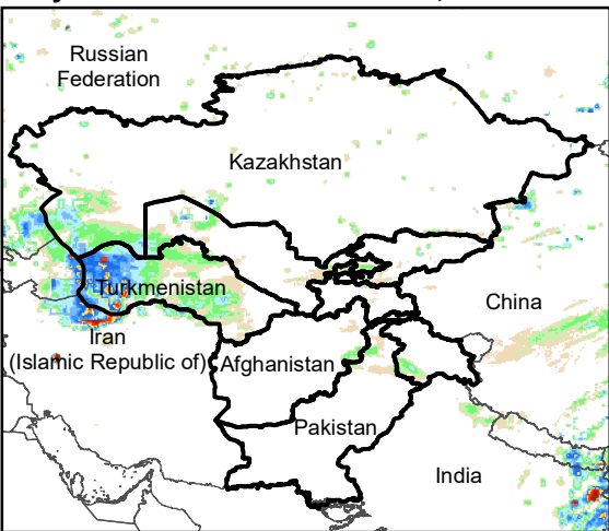
Daily Rainfall estimate for 24 Oct., 2011
