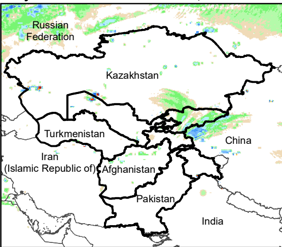
Daily Rainfall estimate for 9 Dec., 2011
