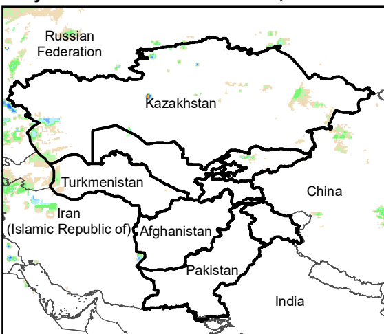
Daily Rainfall estimate for 10 Dec., 2011
