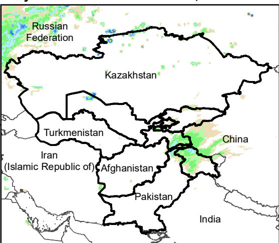
Daily Rainfall estimate for 8 Dec., 2011
