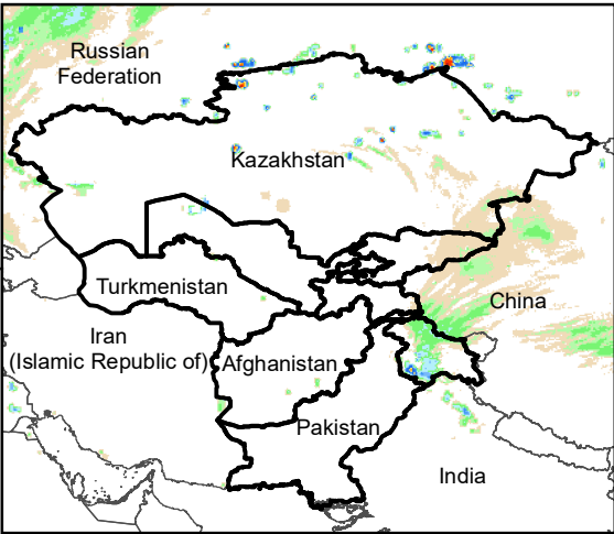
Daily Rainfall estimate for 12 Dec., 2011
