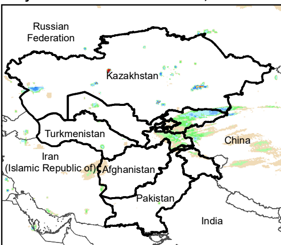
Daily Rainfall estimate for 18 Dec., 2011
