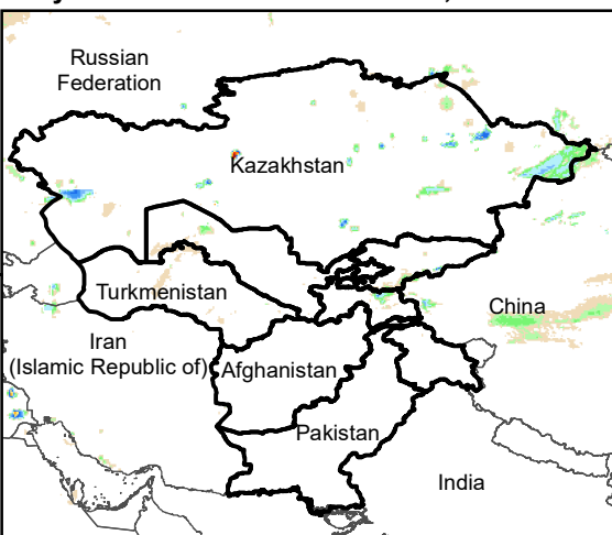
Daily Rainfall estimate for 17 Dec., 2011
