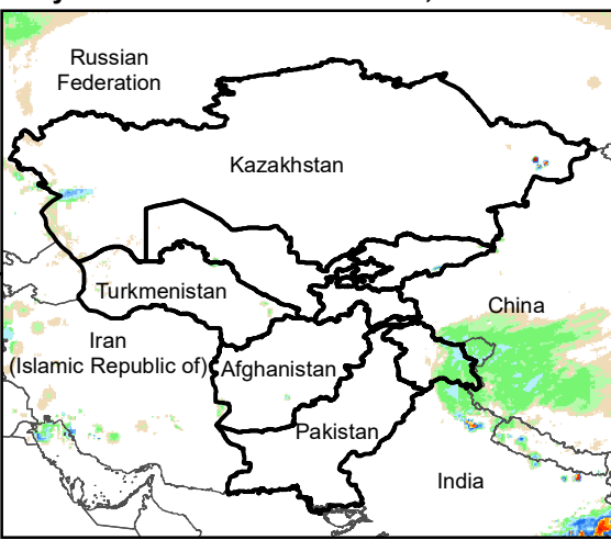
Daily Rainfall estimate for 9 Jan., 2012
