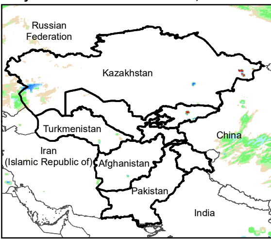
Daily Rainfall estimate for 10 Jan., 2012
