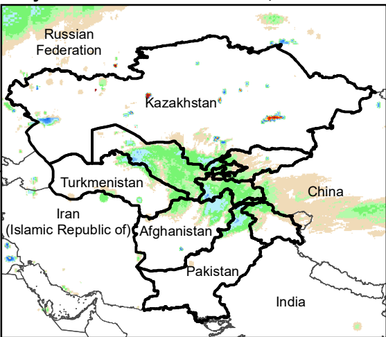
Daily Rainfall estimate for 8 Jan., 2012
